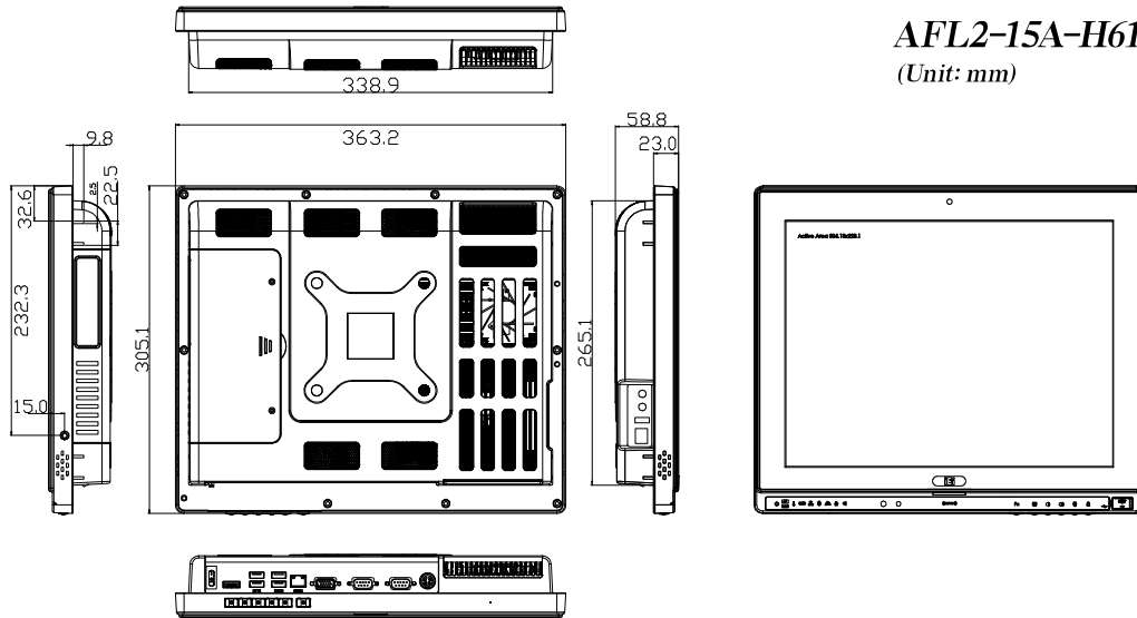
AFL2-W15B-H61 Dimensions (Unit: mm)
